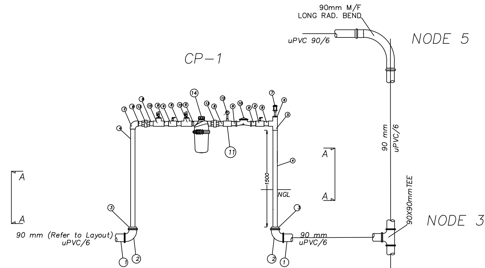
SCHEMATIC SIDE VIEW OF FIELD CONTROL POINTS CP1
