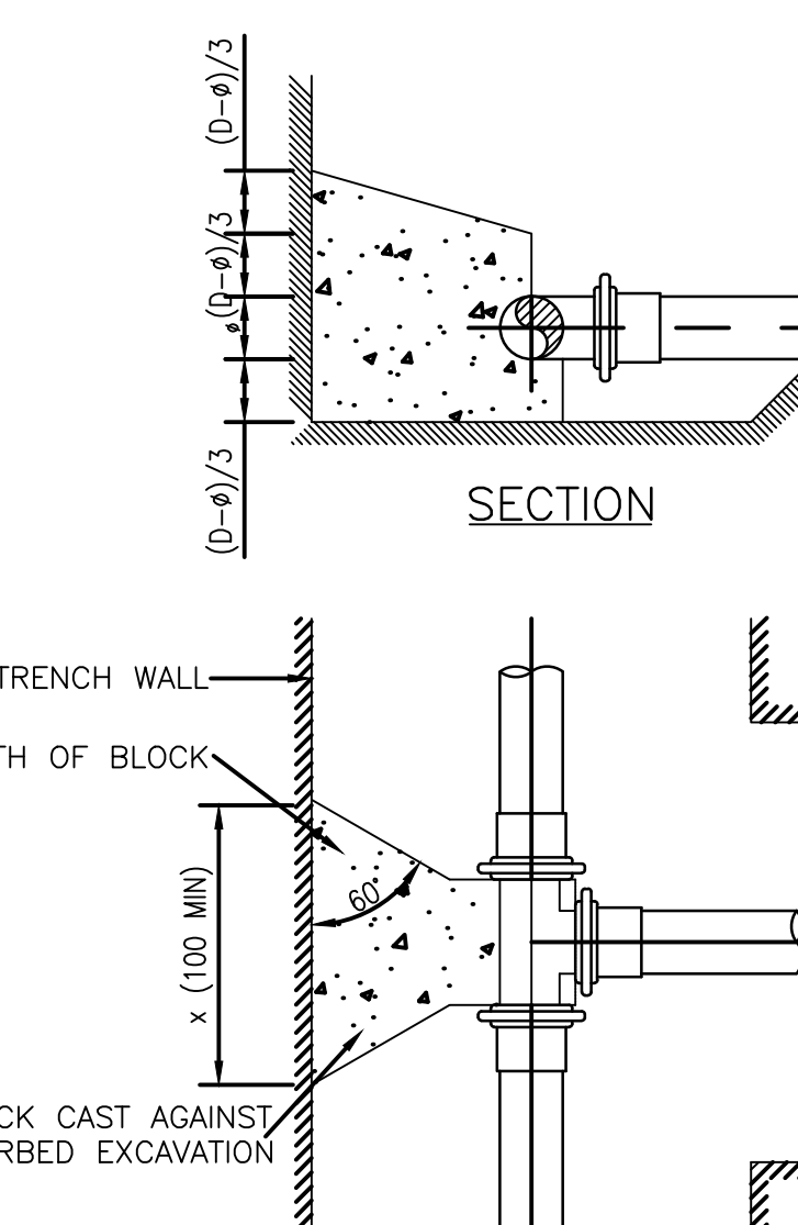
PLAN VIEW OF TEES
