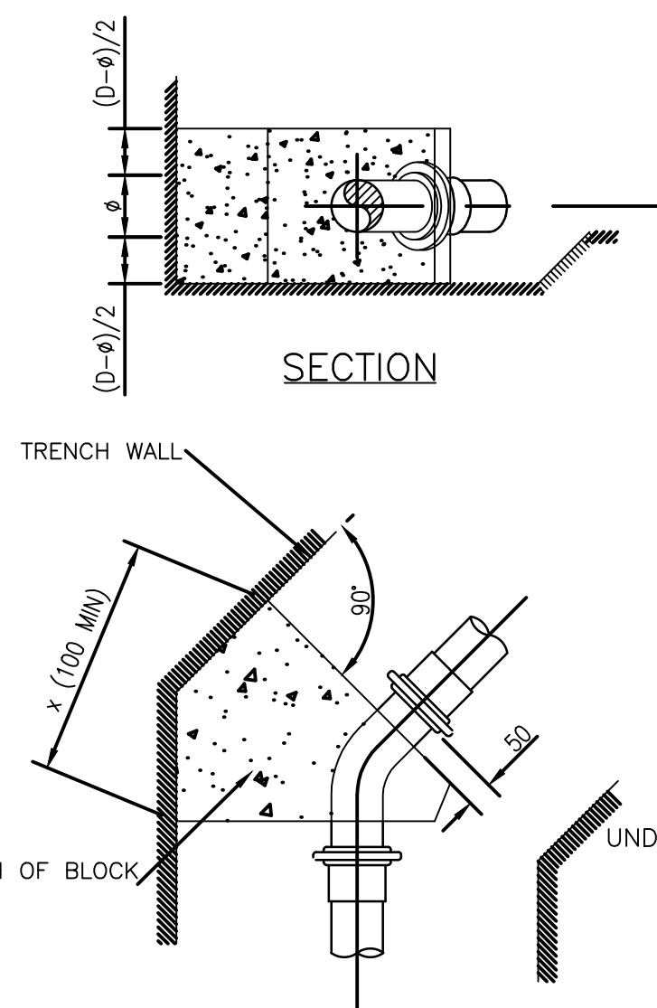
PLAN OF 45° BEND
