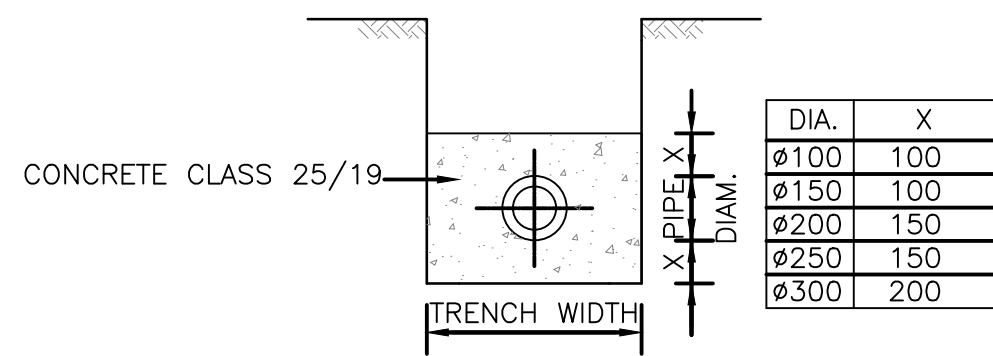
DETAIL OF CONCRETE ENCASUREMENT N.T.S
