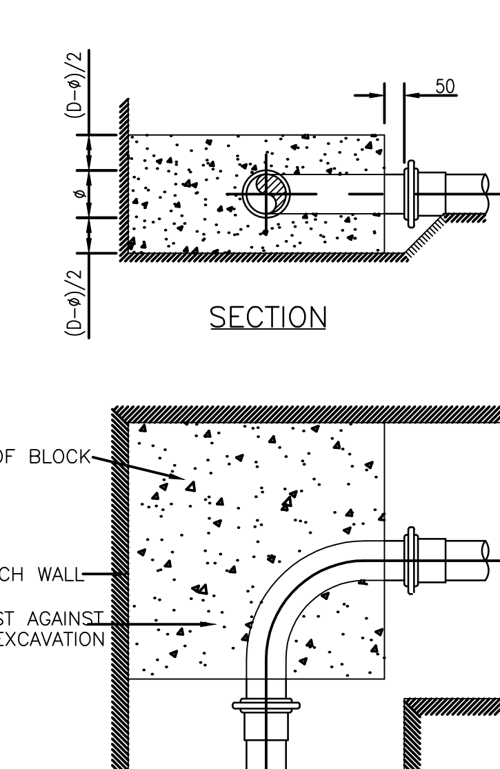
PLAN VIEW OF 90° BEND
